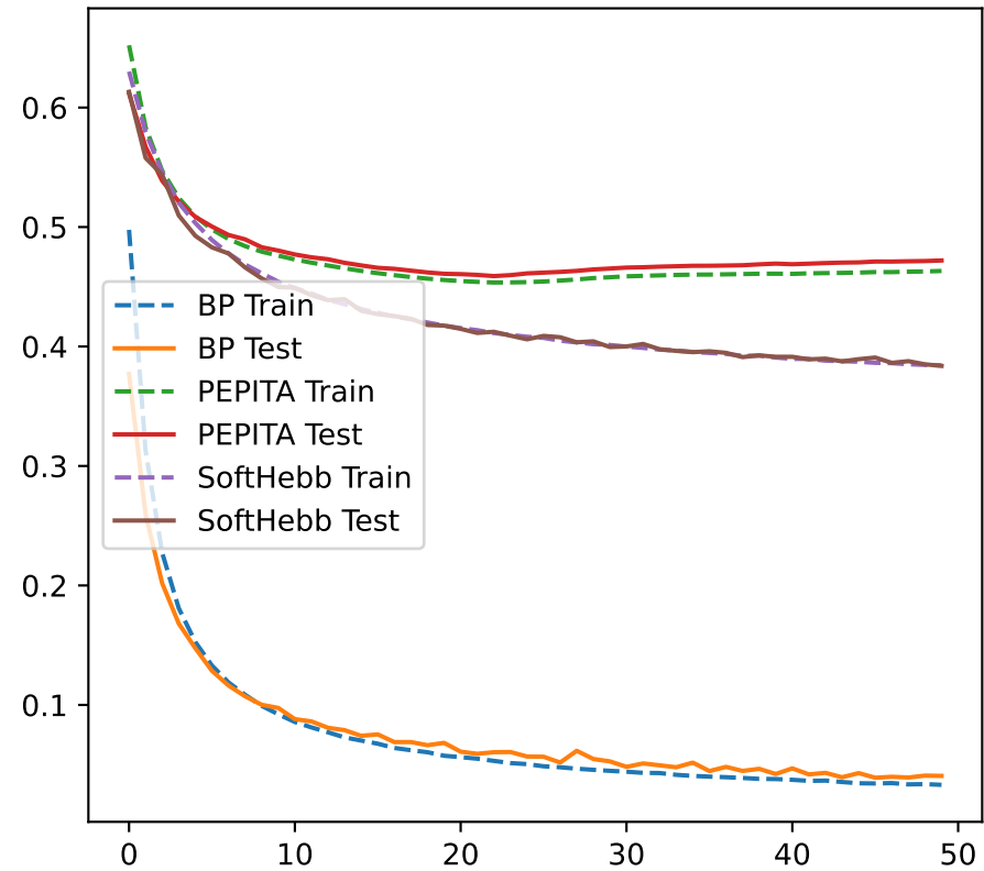
Loss over Epochs
