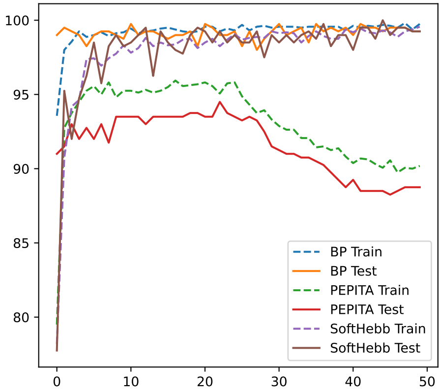
Accuracy over Epochs
